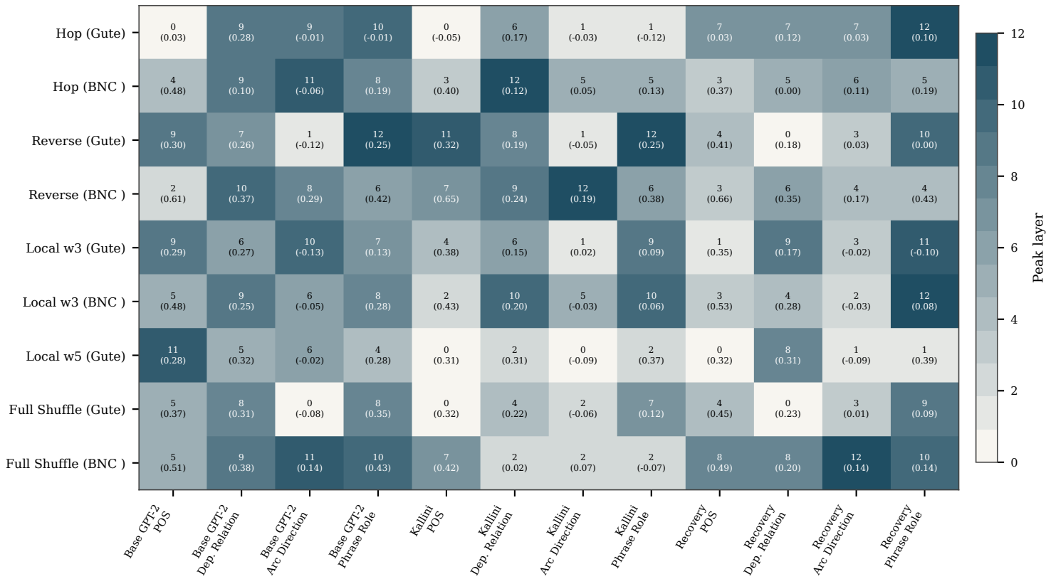
Peak V-information layer (Original)
